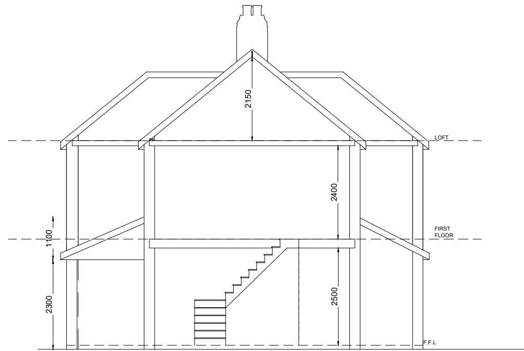
PROPOSED RIGHT SIDE SECTION
